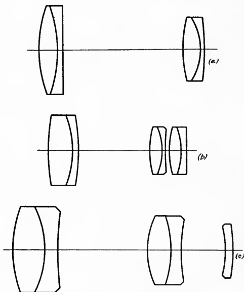
FIG. 3a. Petzval type f/1.6 .
